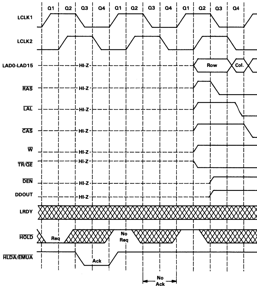
Figure 11-16. TMS34010 Resumes Control of Local Bus
