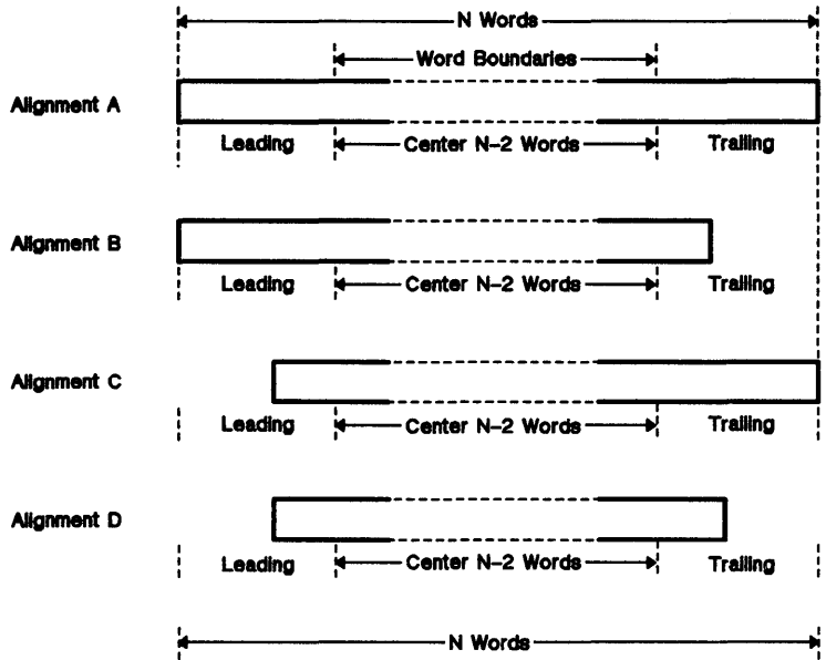
Figure 13-9. Pixel Block Alignments
