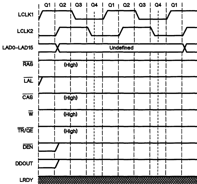
Figure 11-9. Local Bus Internal Cycles Back to Back
