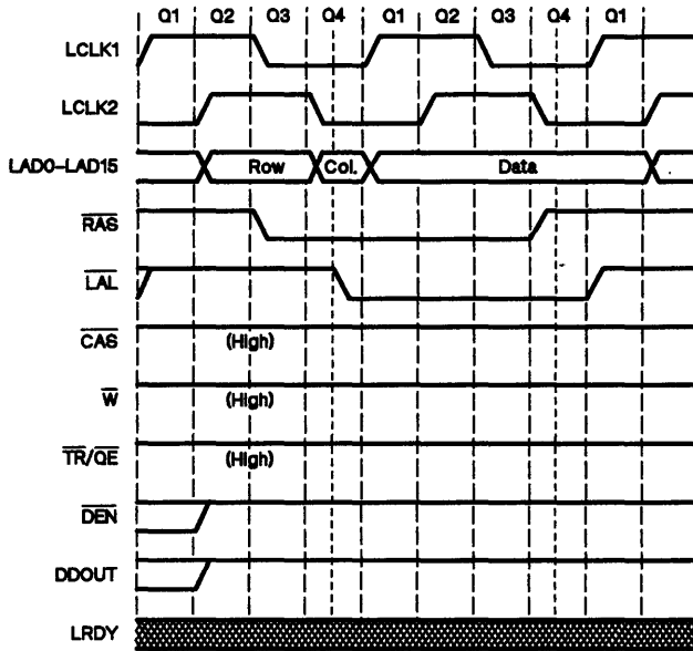
Figure 11-11. I/O Register Write Cycle Timing
