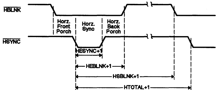
Figure 9-2. Horizontal Timing
