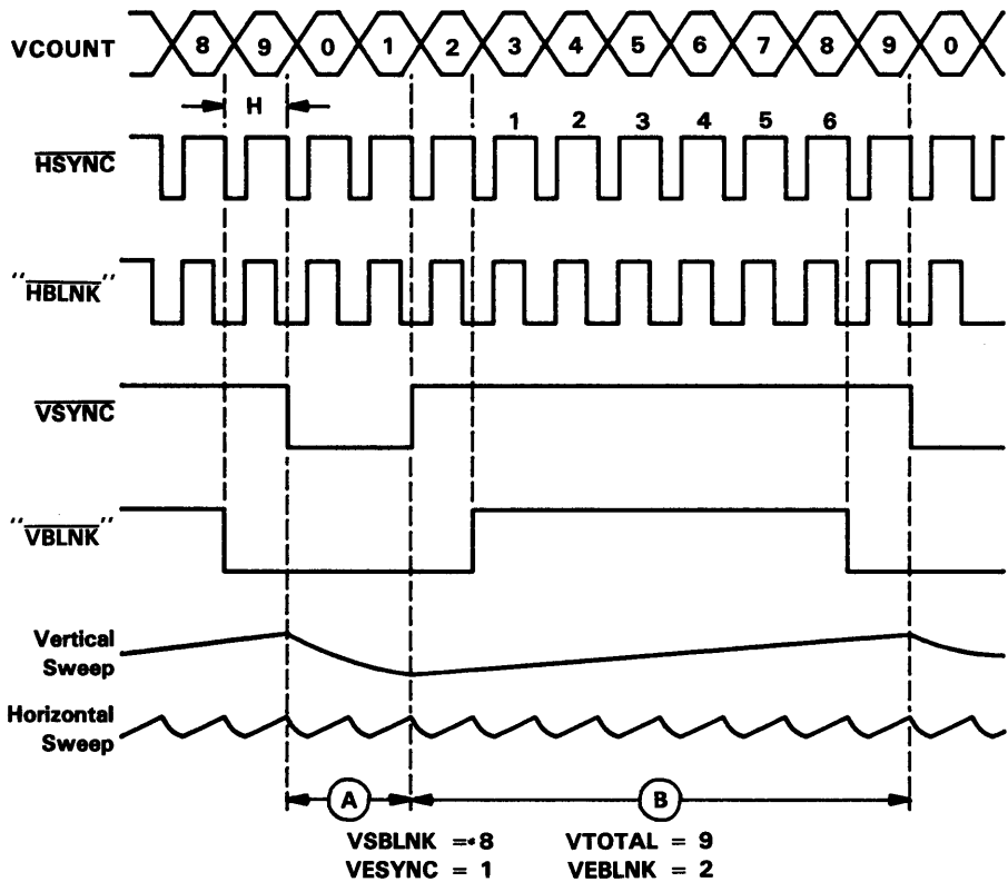
Figure 9-8. Noninterlaced Video Timing Waveform Example
