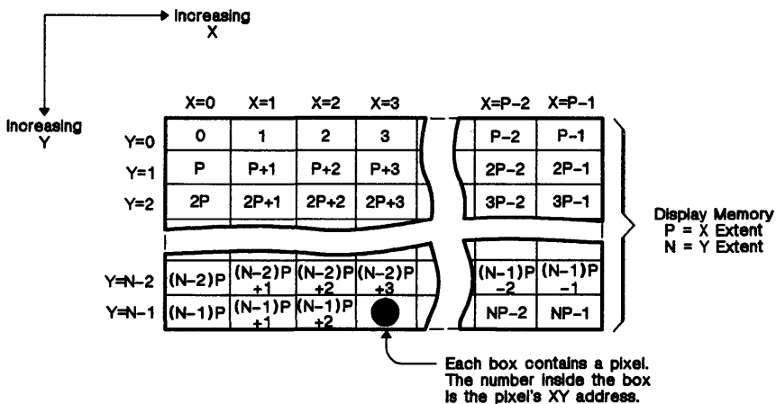
Figure 4-7. Display Memory Dimensions
