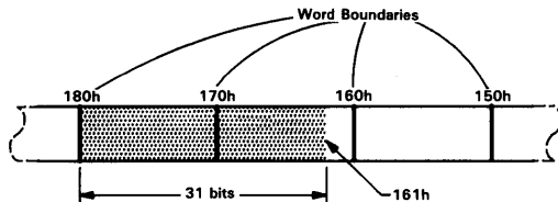
Figure 13-3. Destination Location, Alignment E
