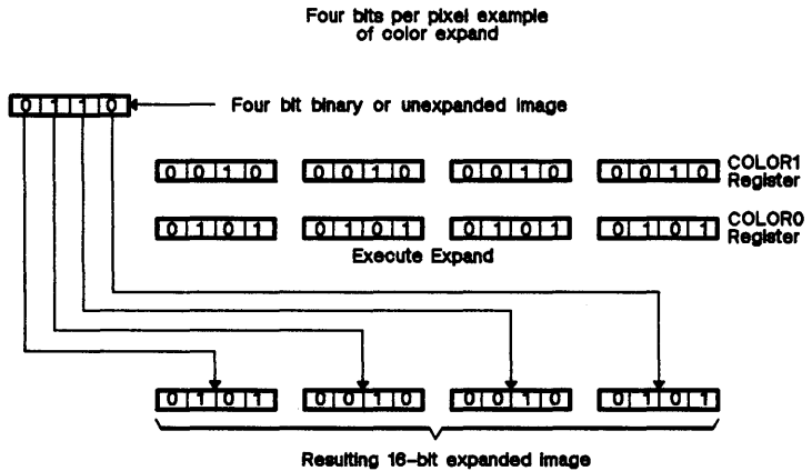
Figure 7-1. Color-Expand Operation
