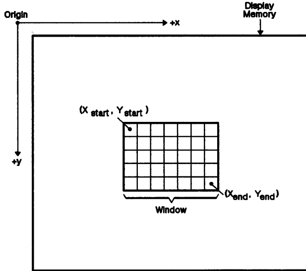
Figure 7-10. Specifying Window Limits
