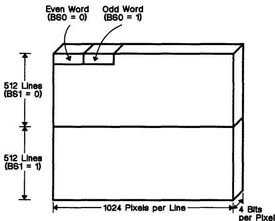
Figure 11-21. Display Memory Dimensions for the Example
