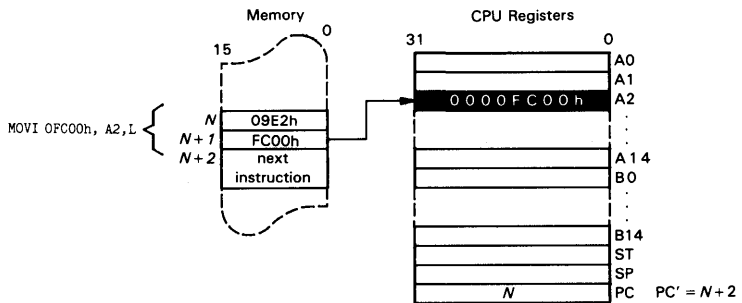
Figure 12-1. An Example of Immediate Addressing
