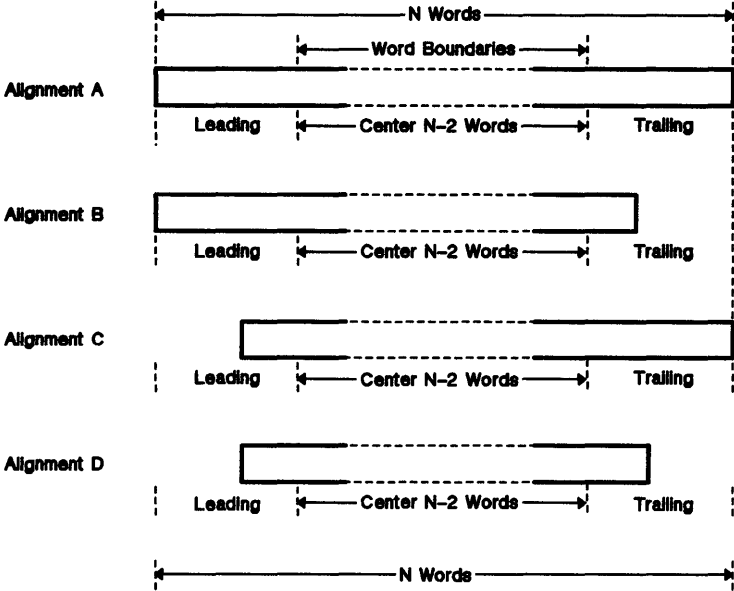
Figure 13-14. Pixel Block Row Alignments
