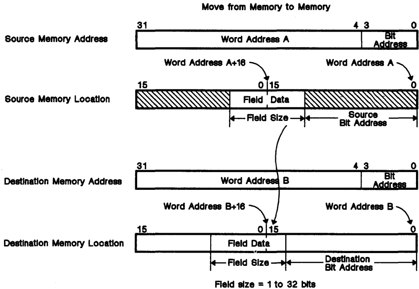
Figure 12-10. Memory-to-Memory Moves
