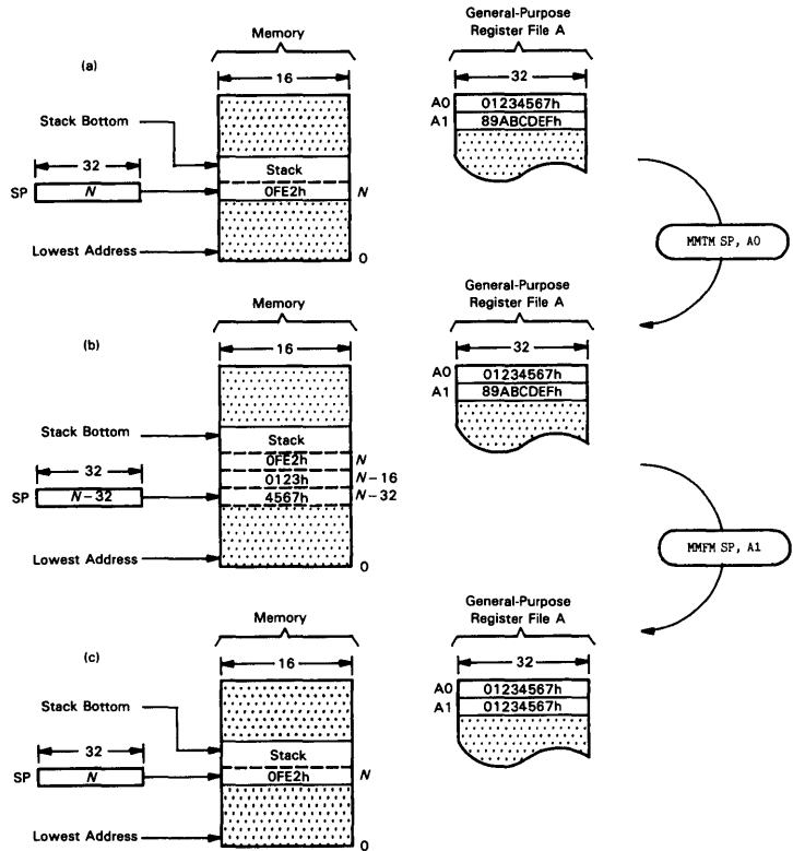
Figure 3-5. Stack Operations
