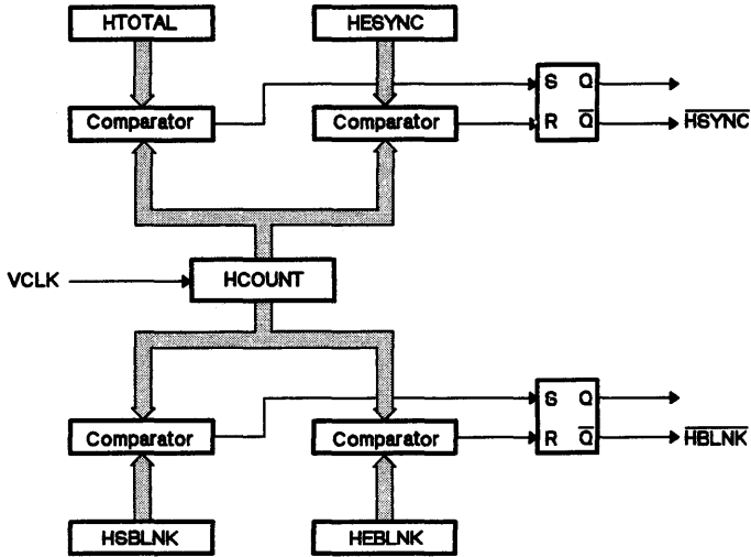
Figure 9-3. Horizontal Timing Logic - Equivalent Circuit
