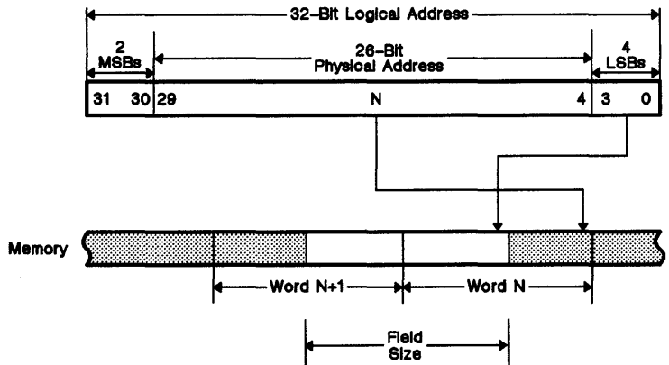
Figure 4-1. Field Storage in External Memory
