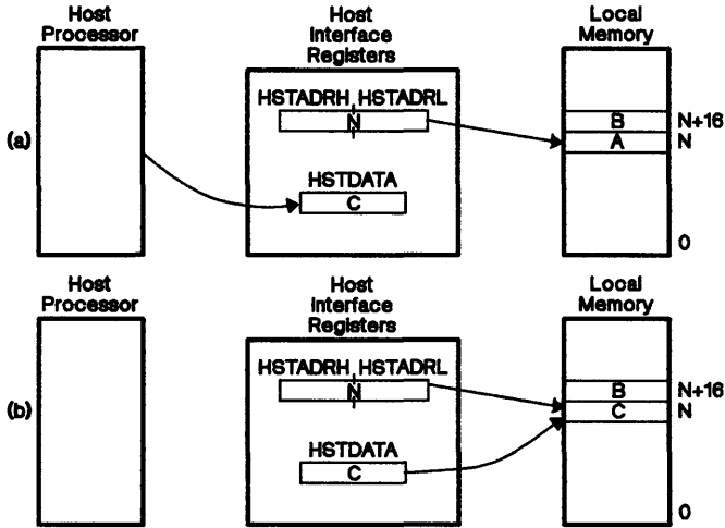
Figure 10-12. Indirect Write Followed by Two Indirect Reads (INCW=1, INCR=0)
