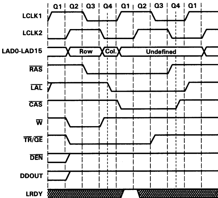
Figure 11-5. Local Bus Register-to-Memory Cycle Timing
