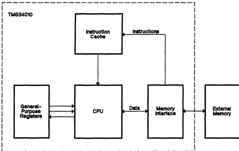
Figure 5-8. Internal Data Paths
