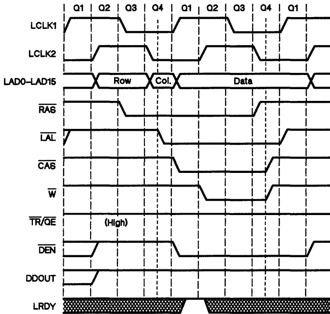
Figure 11-3. Local Bus Write Cycle Timing
