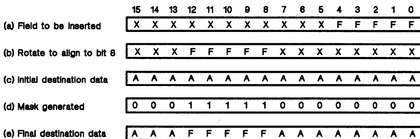
Figure 4-3. Field Insertion
